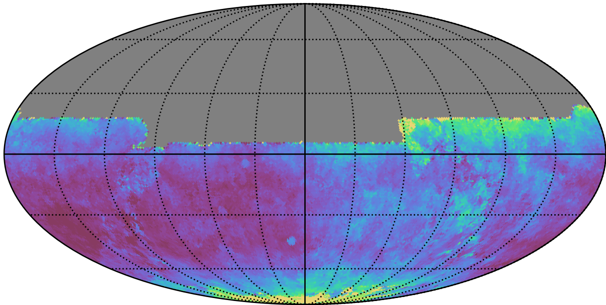
too_elab_r16_d3_gz_v3.4_10yrs All sky y band: Median seeingEff
