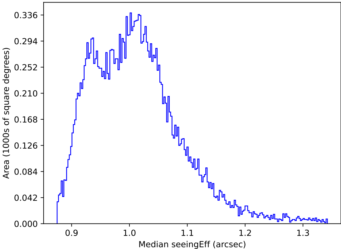
too_elab_r16_d3_gz_v3.4_10yrs All sky y band: Median seeingEff
