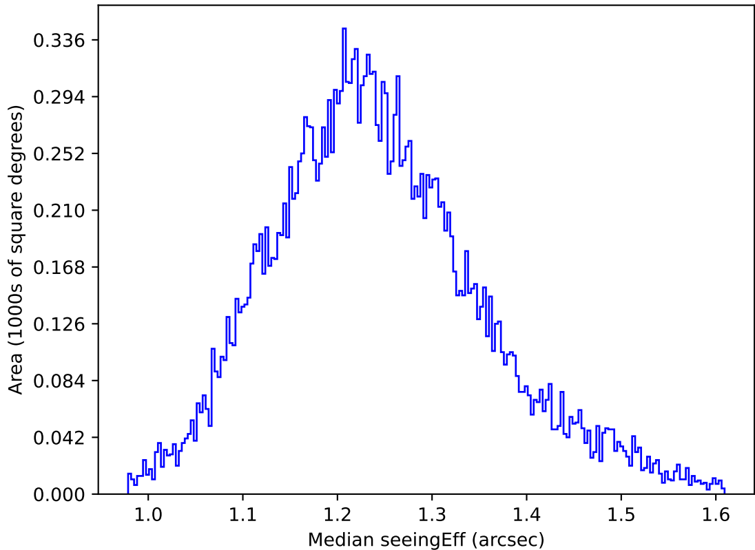
too_elab_r16_d3_gz_v3.4_10yrs All sky u band: Median seeingEff
