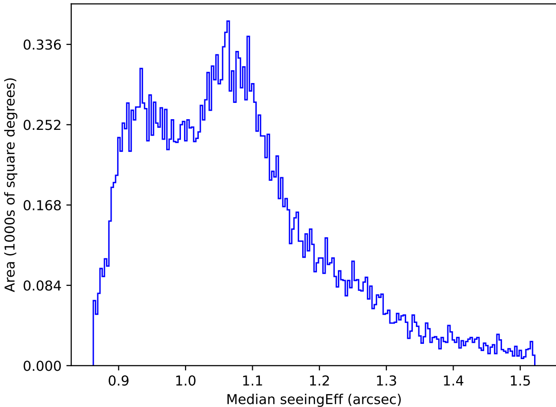
too_elab_r16_d3_gz_v3.4_10yrs All sky r band: Median seeingEff
