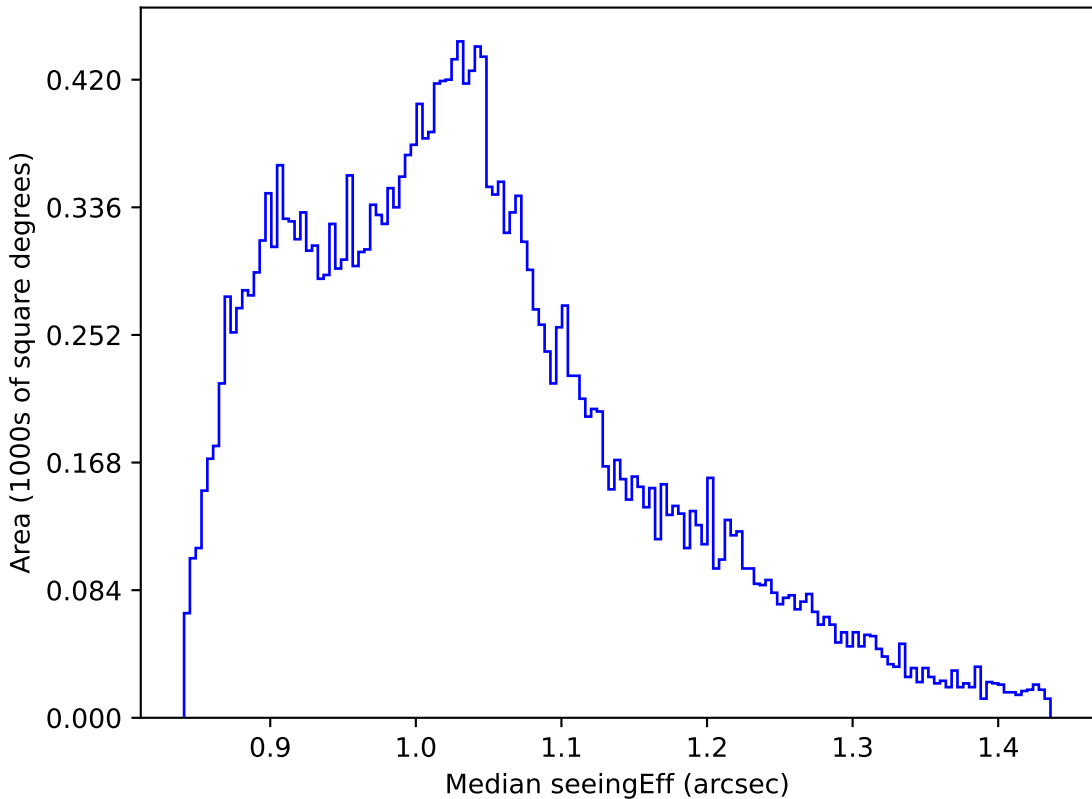
too_elab_r16_d3_gz_v3.4_10yrs All sky i band: Median seeingEff
