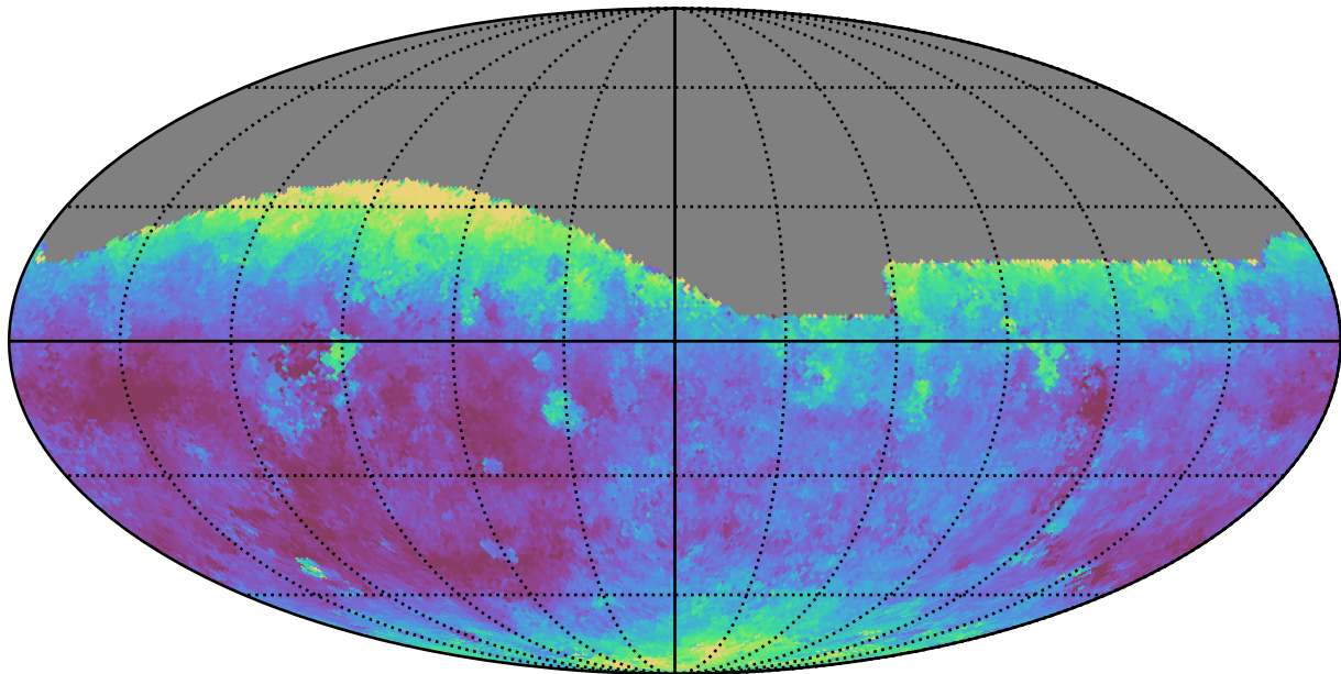
too_elab_r16_d3_gz_v3.4_10yrs All sky g band: Median seeingEff
