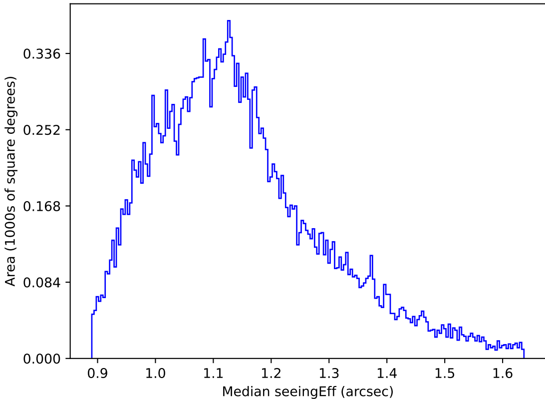
too_elab_r16_d3_gz_v3.4_10yrs All sky g band: Median seeingEff
