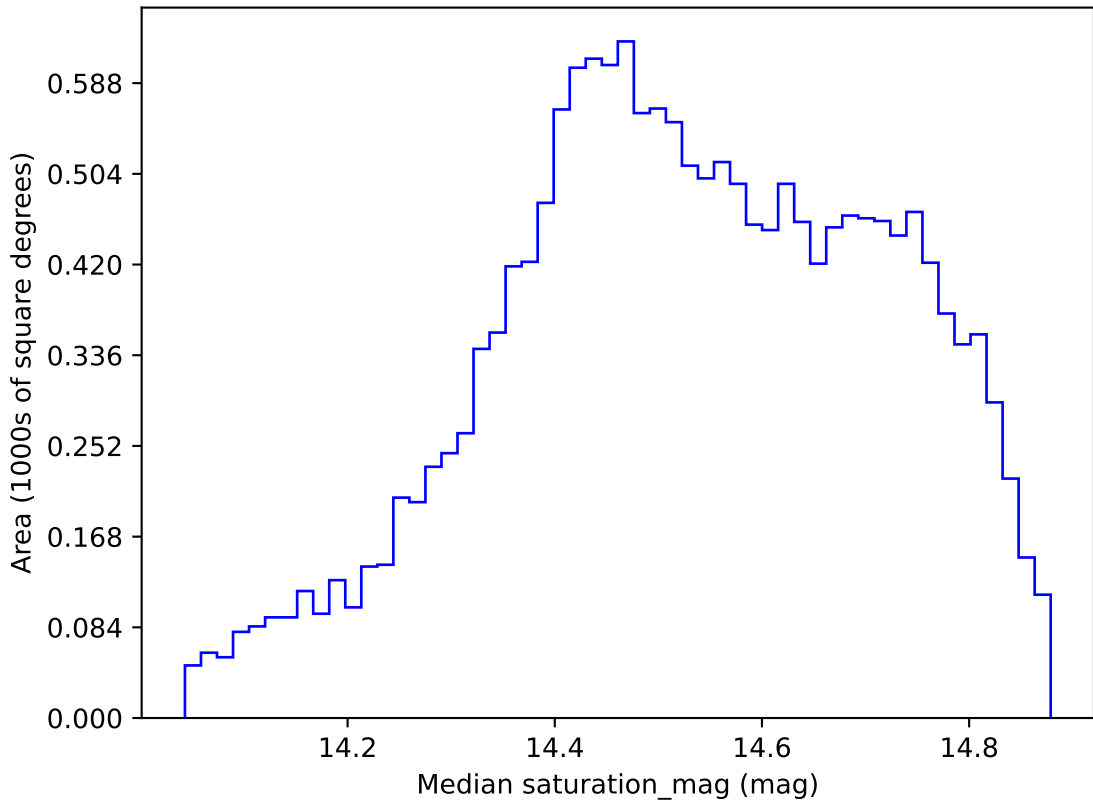
too_elab_r16_d3_gz_v3.4_10yrs WFD i band: Median saturation_mag
