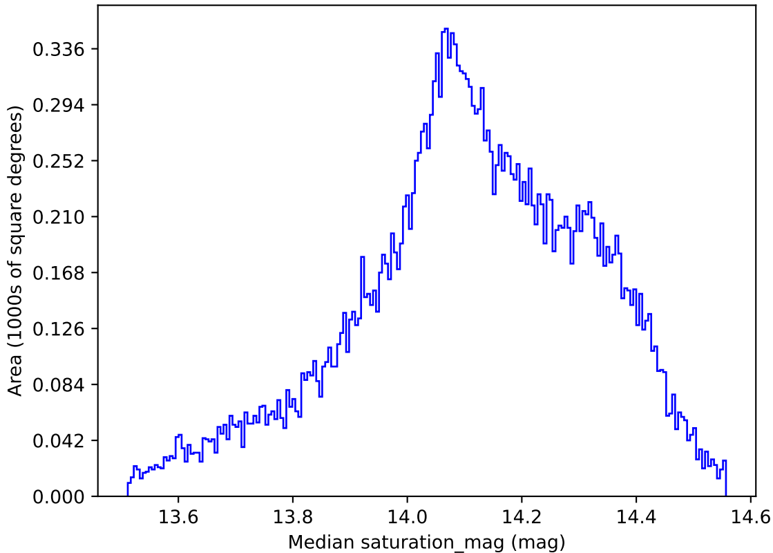
too_elab_r16_d3_gz_v3.4_10yrs All sky all bands: Median saturation_mag
