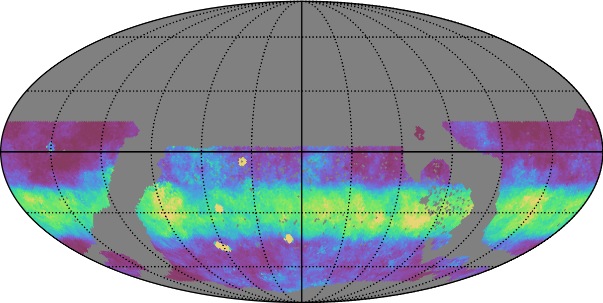
too_elab_r16_d3_gz_v3.4_10yrs WFD z band: Median normairmass
