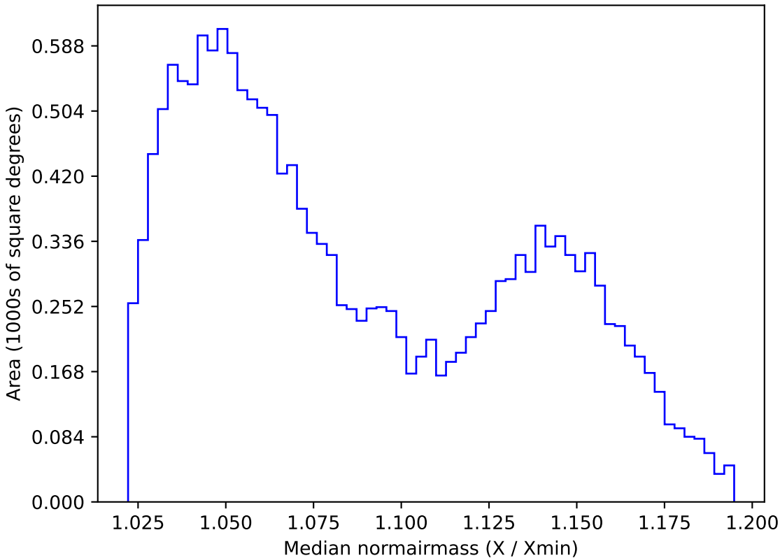
too_elab_r16_d3_gz_v3.4_10yrs WFD z band: Median normairmass
