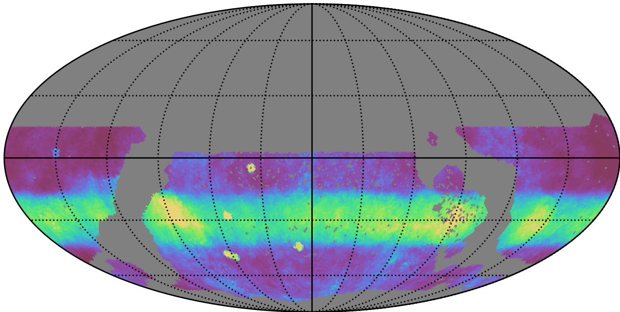
too_elab_r16_d3_gz_v3.4_10yrs WFD r band: Median normairmass
