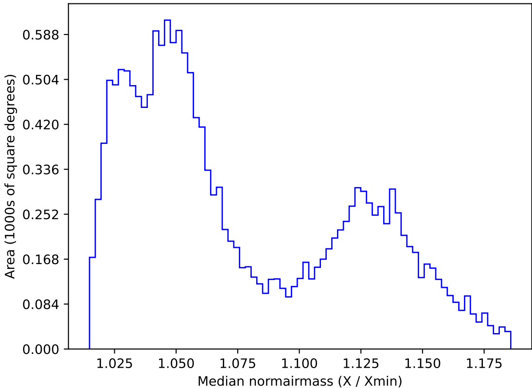
too_elab_r16_d3_gz_v3.4_10yrs WFD r band: Median normairmass
