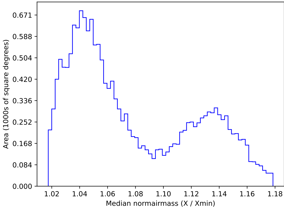
too_elab_r16_d3_gz_v3.4_10yrs WFD i band: Median normairmass
