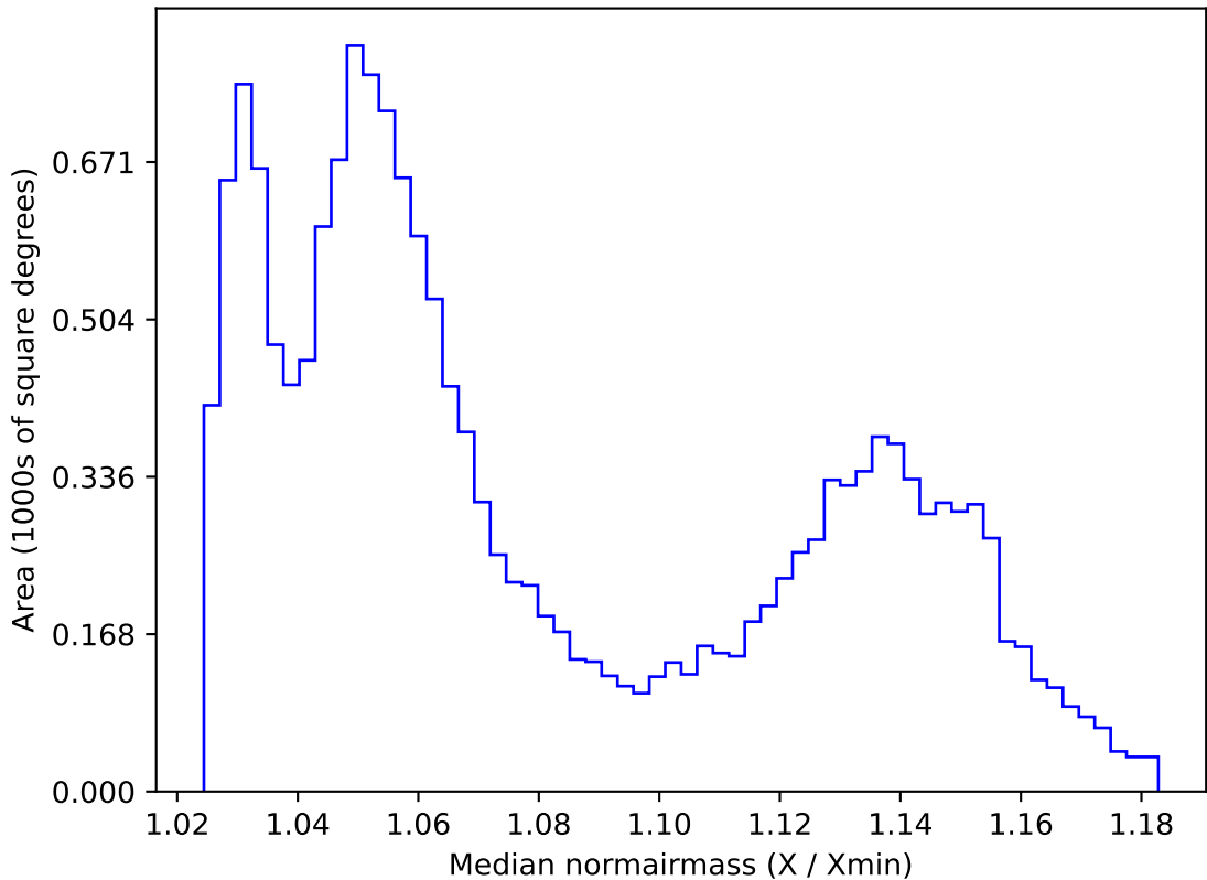
too_elab_r16_d3_gz_v3.4_10yrs WFD all bands: Median normairmass
