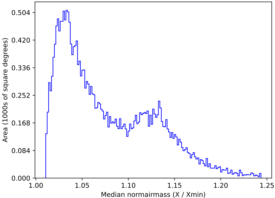
too_elab_r16_d3_gz_v3.4_10yrs All sky u band: Median normairmass
