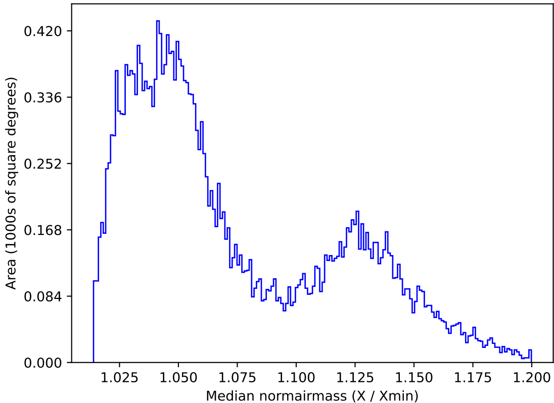
too_elab_r16_d3_gz_v3.4_10yrs All sky r band: Median normairmass
