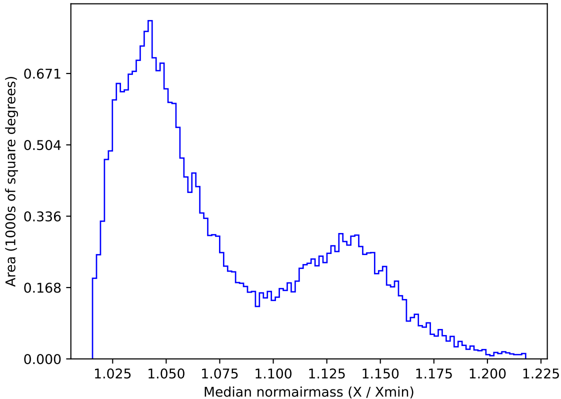
too_elab_r16_d3_gz_v3.4_10yrs All sky i band: Median normairmass
