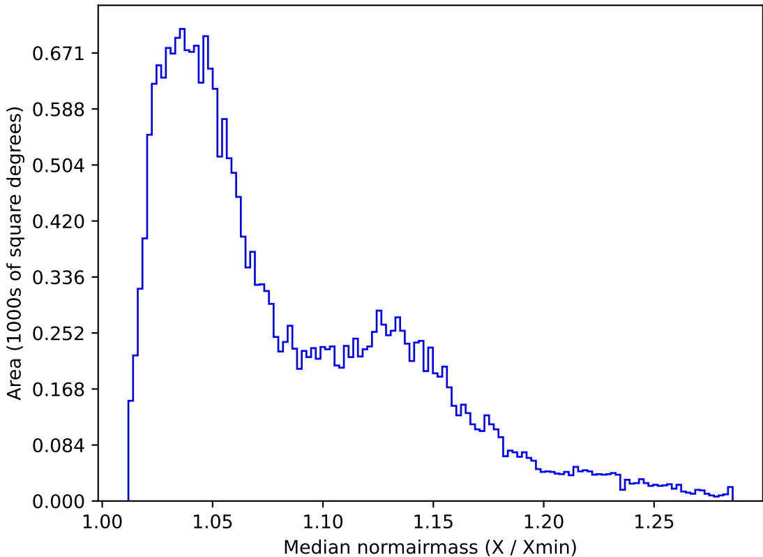
too_elab_r16_d3_gz_v3.4_10yrs All sky g band: Median normairmass
