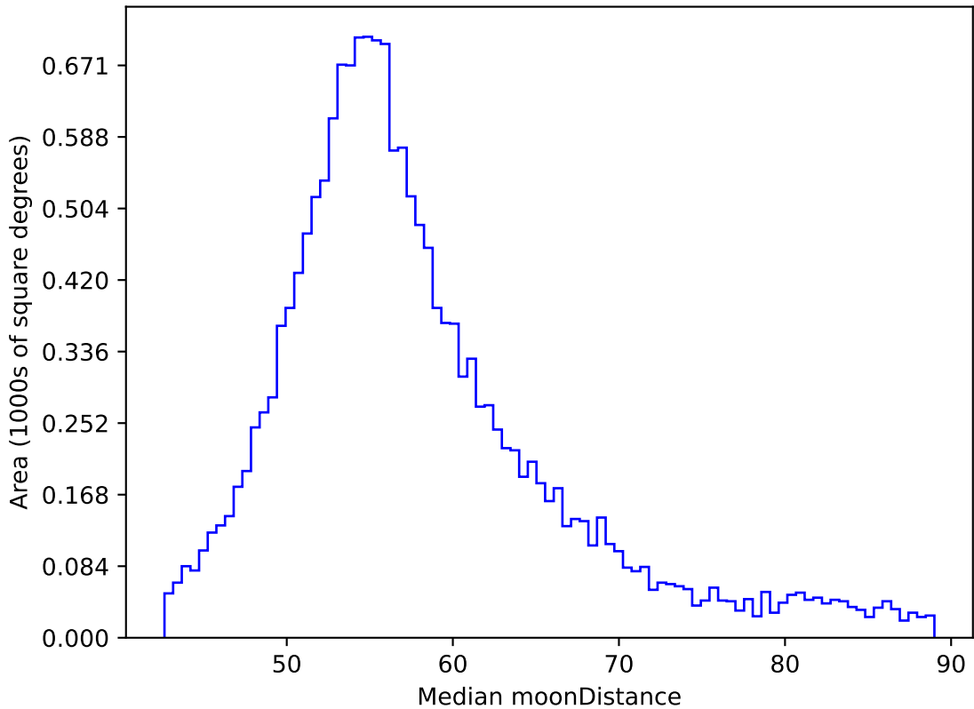
too_elab_r16_d3_gz_v3.4_10yrs WFD y band: Median moonDistance
