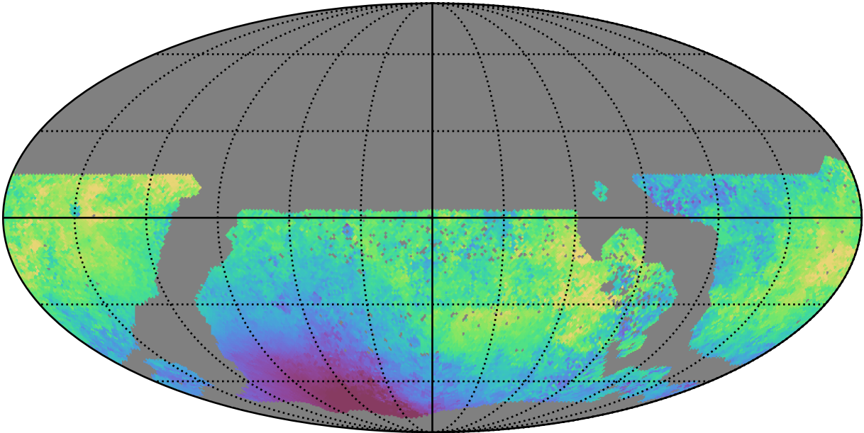
too_elab_r16_d3_gz_v3.4_10yrs WFD u band: Median moonDistance
