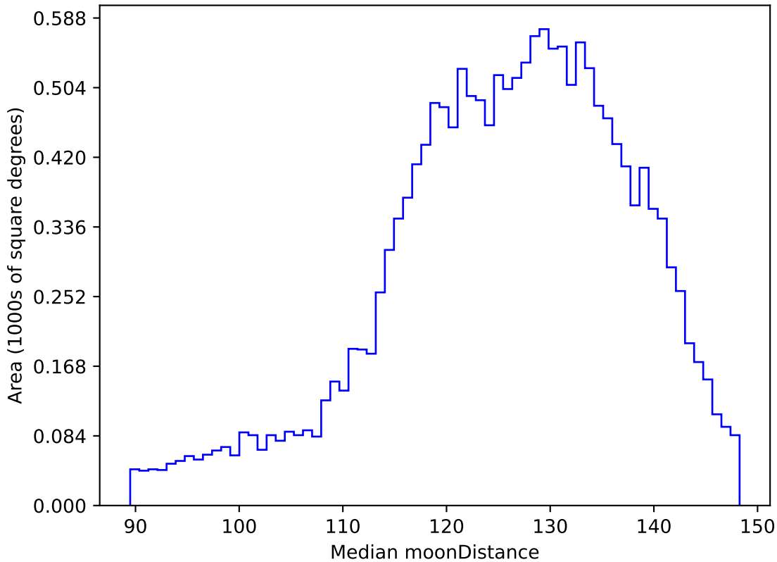
too_elab_r16_d3_gz_v3.4_10yrs WFD u band: Median moonDistance
