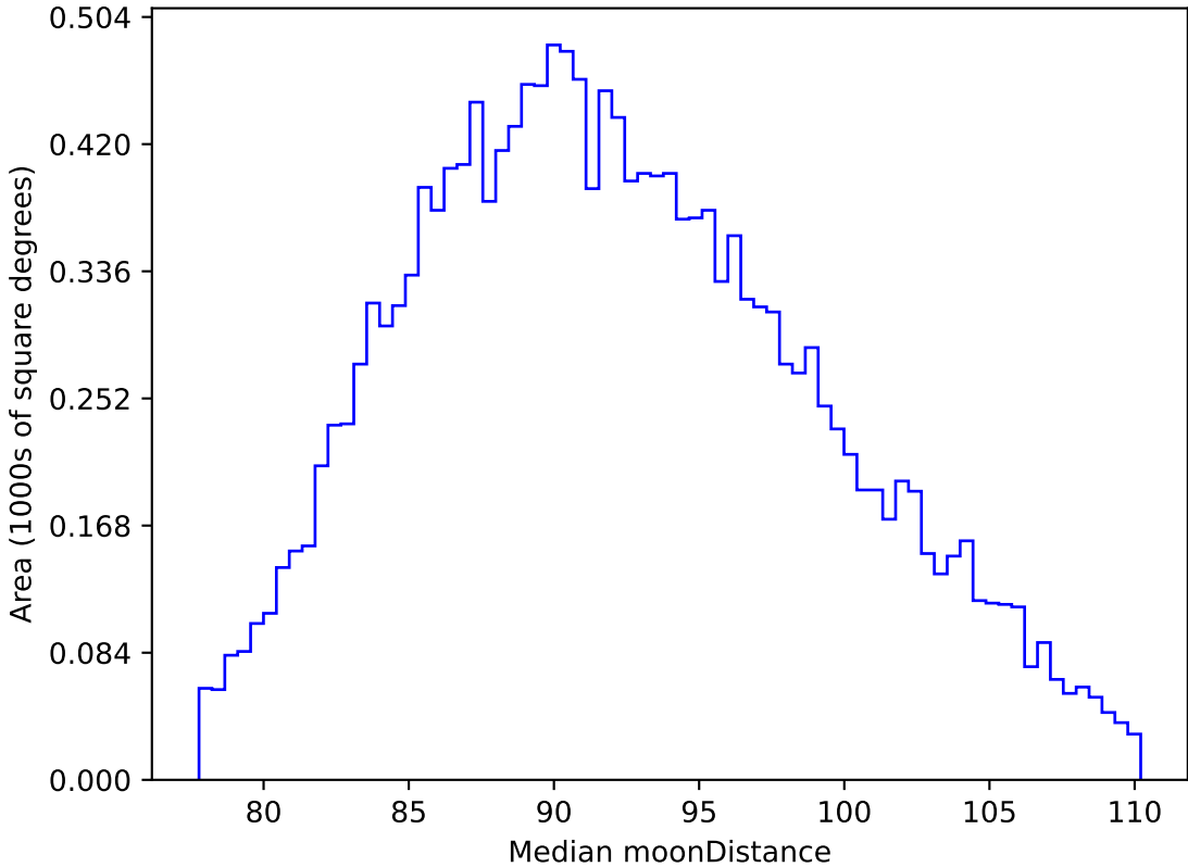
too_elab_r16_d3_gz_v3.4_10yrs WFD i band: Median moonDistance
