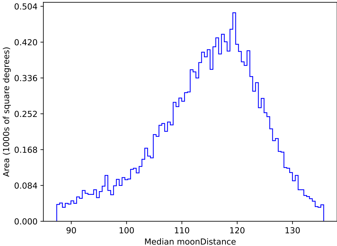
too_elab_r16_d3_gz_v3.4_10yrs WFD g band: Median moonDistance
