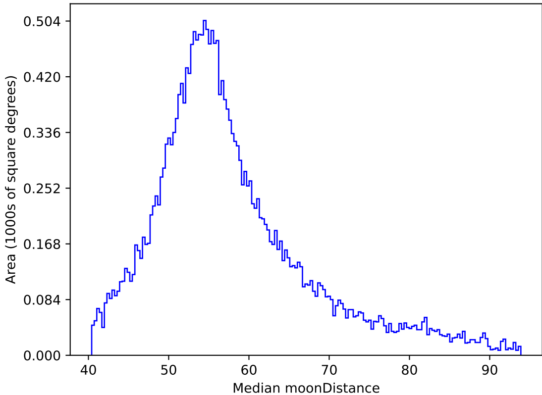
too_elab_r16_d3_gz_v3.4_10yrs All sky y band: Median moonDistance
