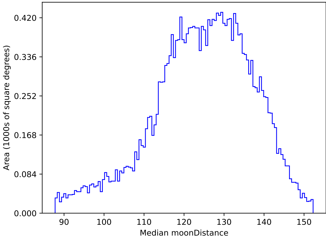
too_elab_r16_d3_gz_v3.4_10yrs All sky u band: Median moonDistance
