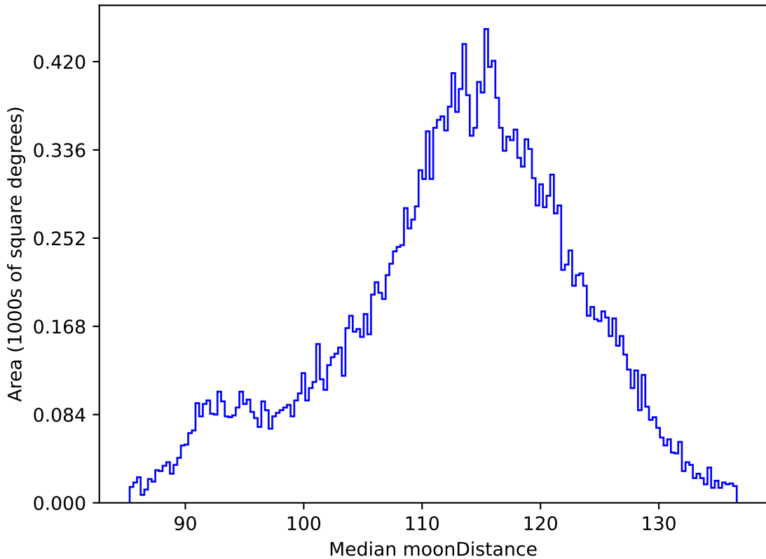
too_elab_r16_d3_gz_v3.4_10yrs All sky r band: Median moonDistance
