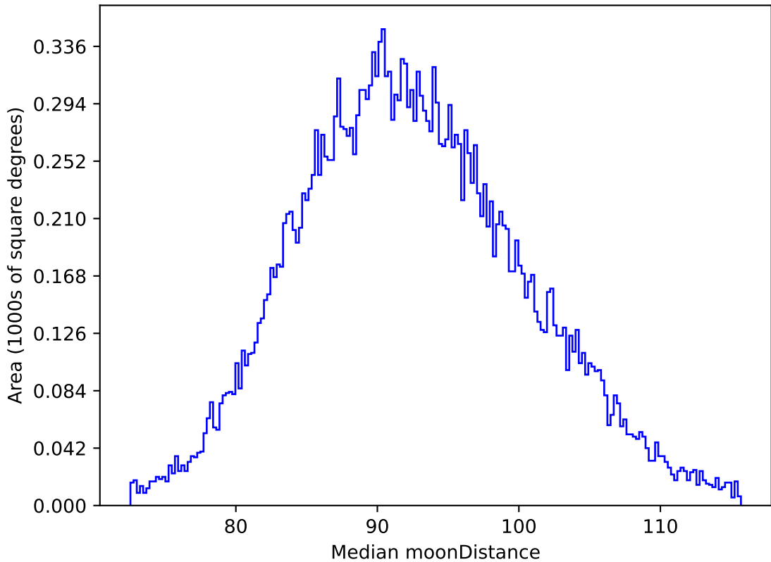
too_elab_r16_d3_gz_v3.4_10yrs All sky i band: Median moonDistance
