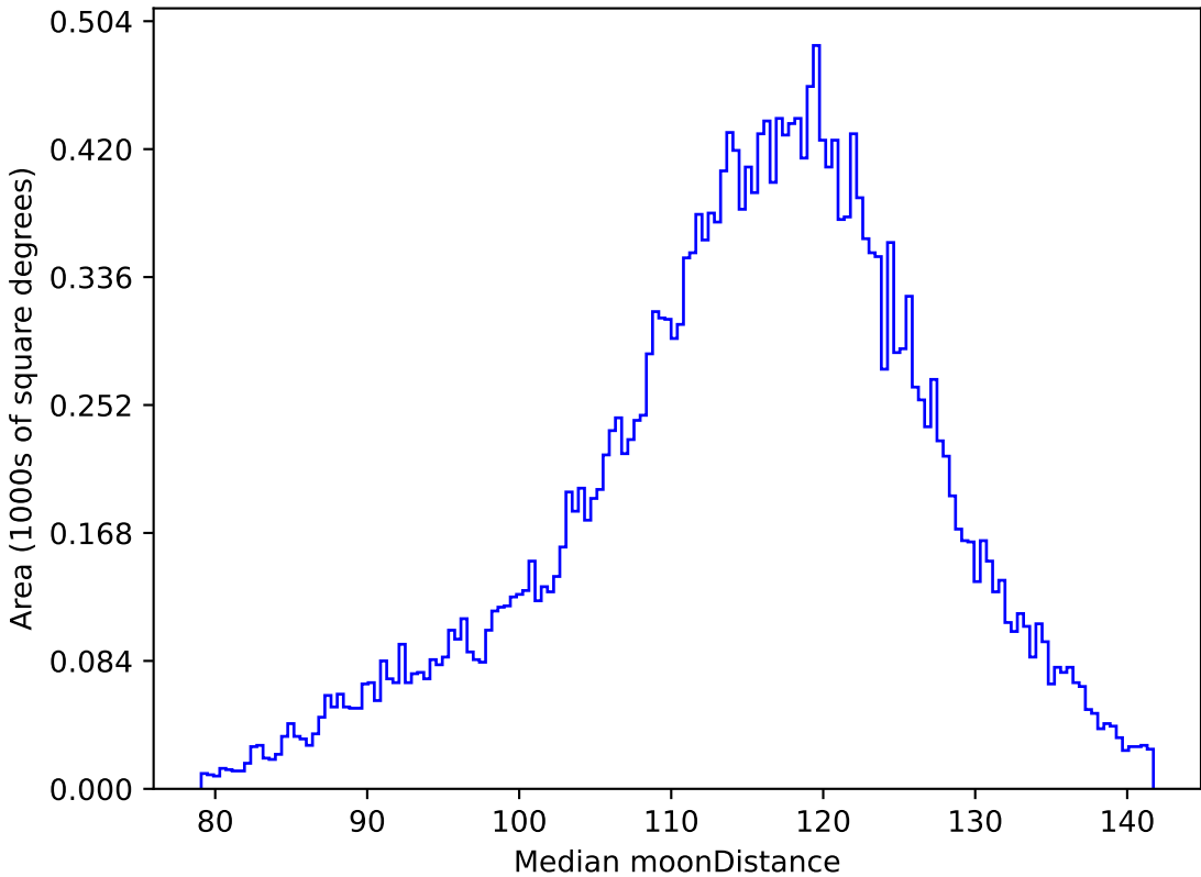
too_elab_r16_d3_gz_v3.4_10yrs All sky g band: Median moonDistance
