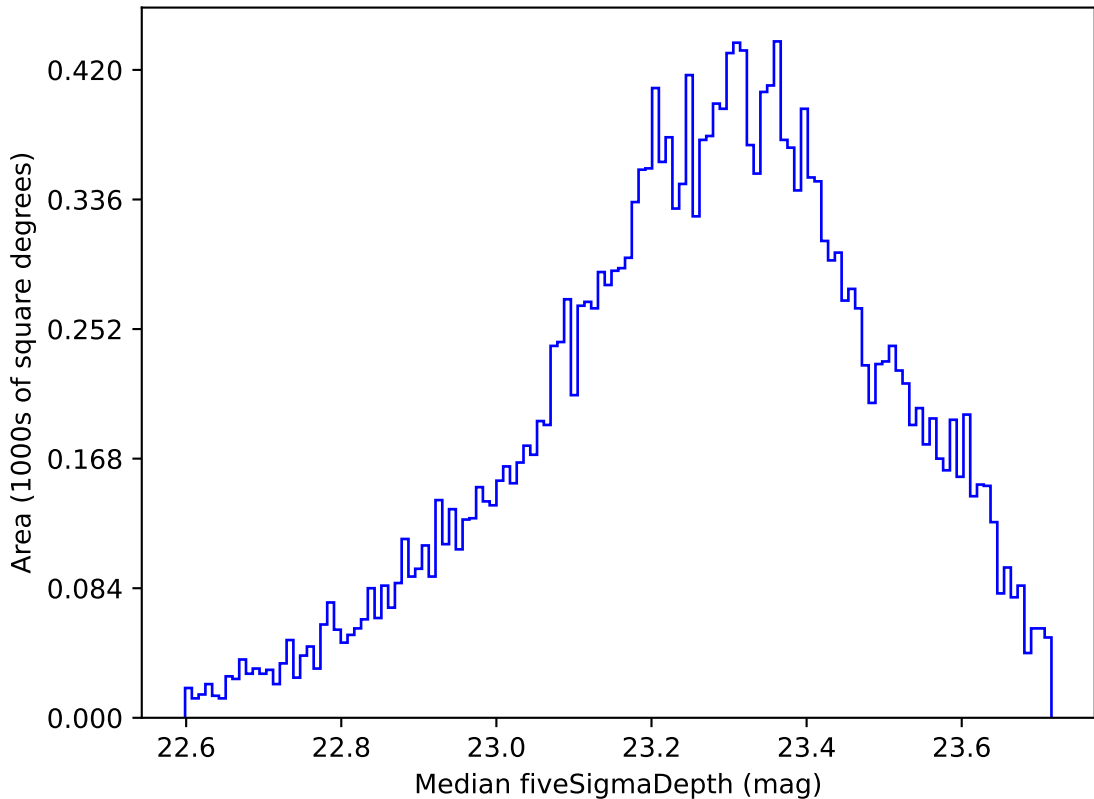
too_elab_r16_d3_gz_v3.4_10yrs Yr 1 u band: Median fiveSigmaDepth
