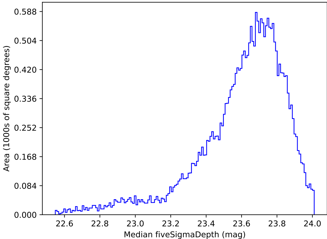
too_elab_r16_d3_gz_v3.4_10yrs Yr 1 i band: Median fiveSigmaDepth
