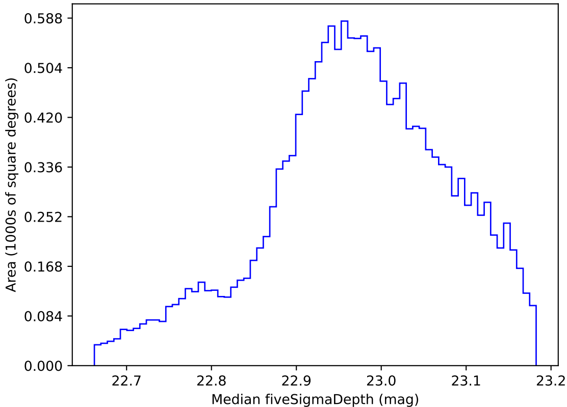
too_elab_r16_d3_gz_v3.4_10yrs WFD z band: Median fiveSigmaDepth
