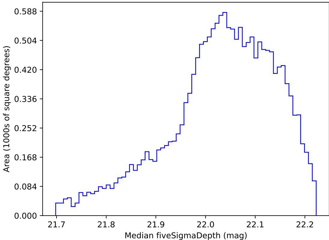
too_elab_r16_d3_gz_v3.4_10yrs WFD y band: Median fiveSigmaDepth
