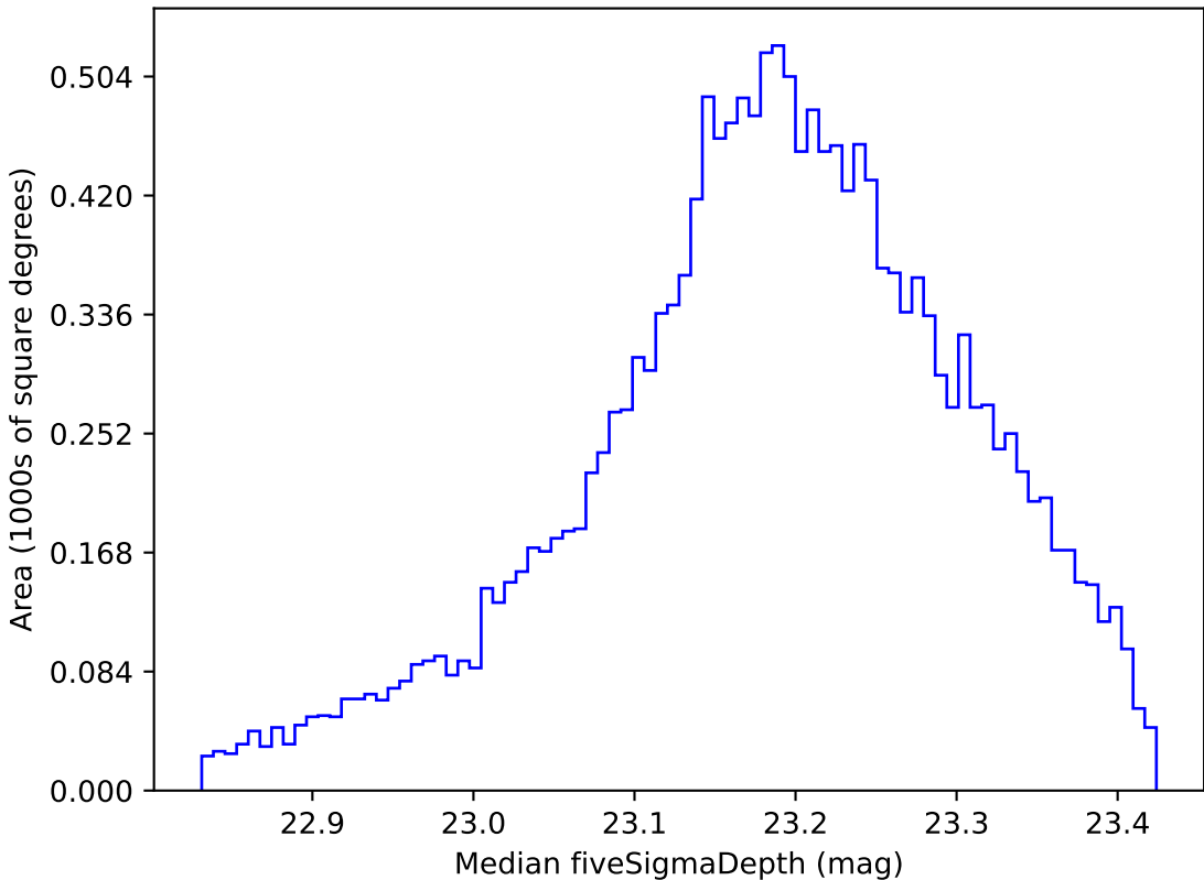
too_elab_r16_d3_gz_v3.4_10yrs WFD u band: Median fiveSigmaDepth
