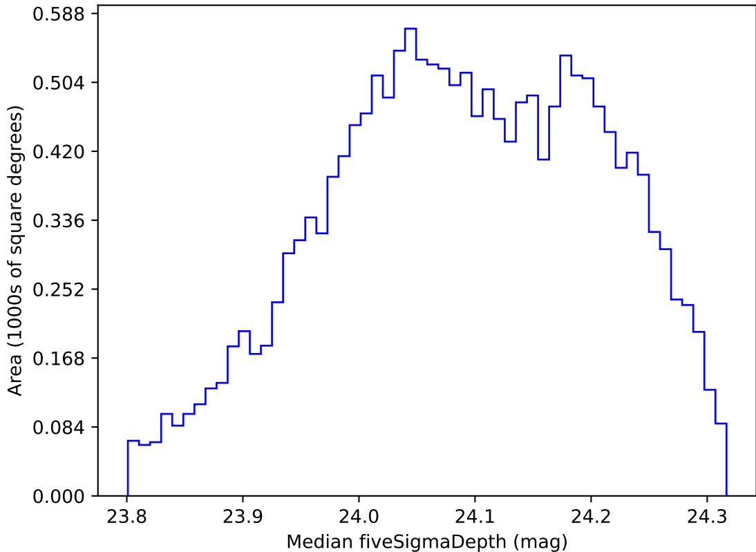
too_elab_r16_d3_gz_v3.4_10yrs WFD r band: Median fiveSigmaDepth
