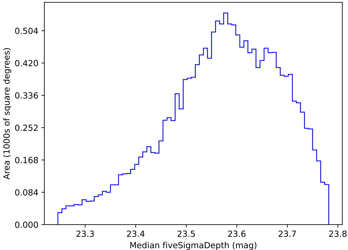
too_elab_r16_d3_gz_v3.4_10yrs WFD i band: Median fiveSigmaDepth
