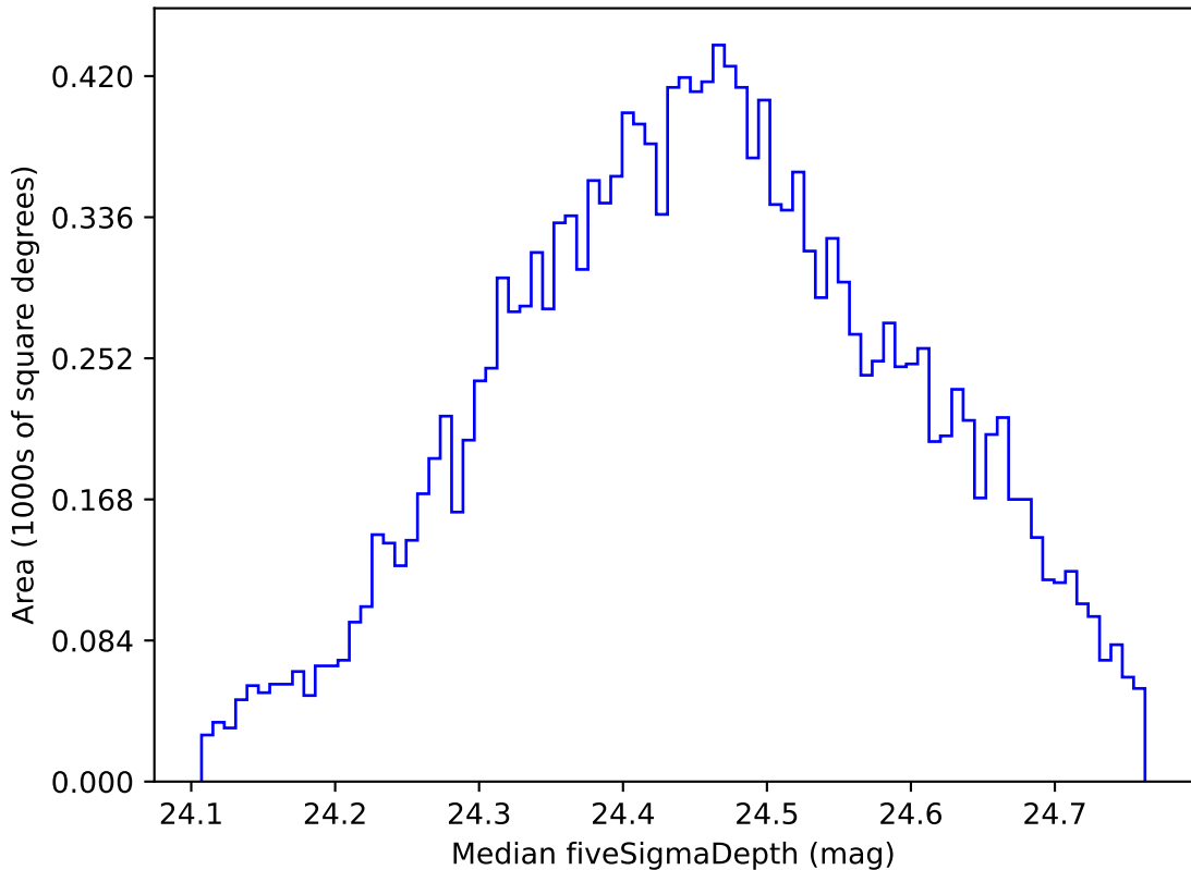
too_elab_r16_d3_gz_v3.4_10yrs WFD g band: Median fiveSigmaDepth
