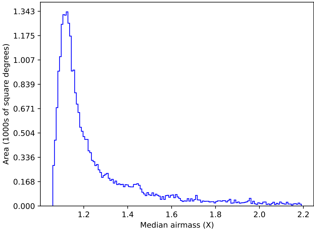
too_elab_r16_d3_gz_v3.4_10yrs Yr 1 z band: Median airmass
