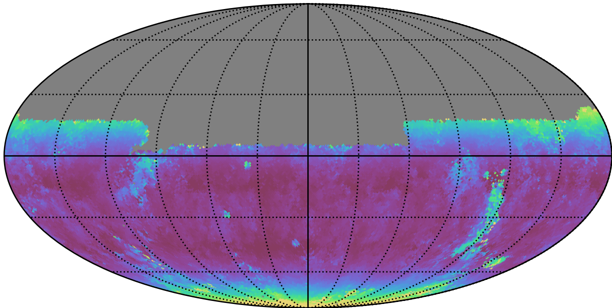
too_elab_r16_d3_gz_v3.4_10yrs Yr 1 y band: Median airmass
