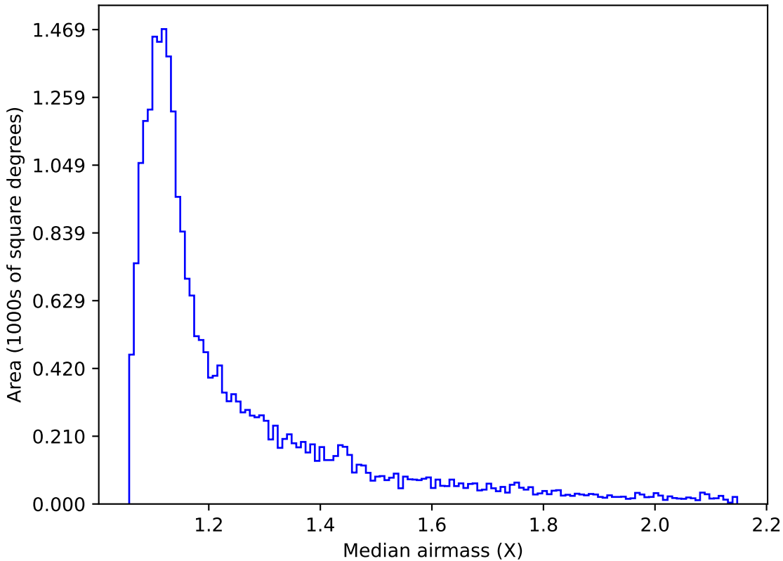
too_elab_r16_d3_gz_v3.4_10yrs Yr 1 r band: Median airmass
