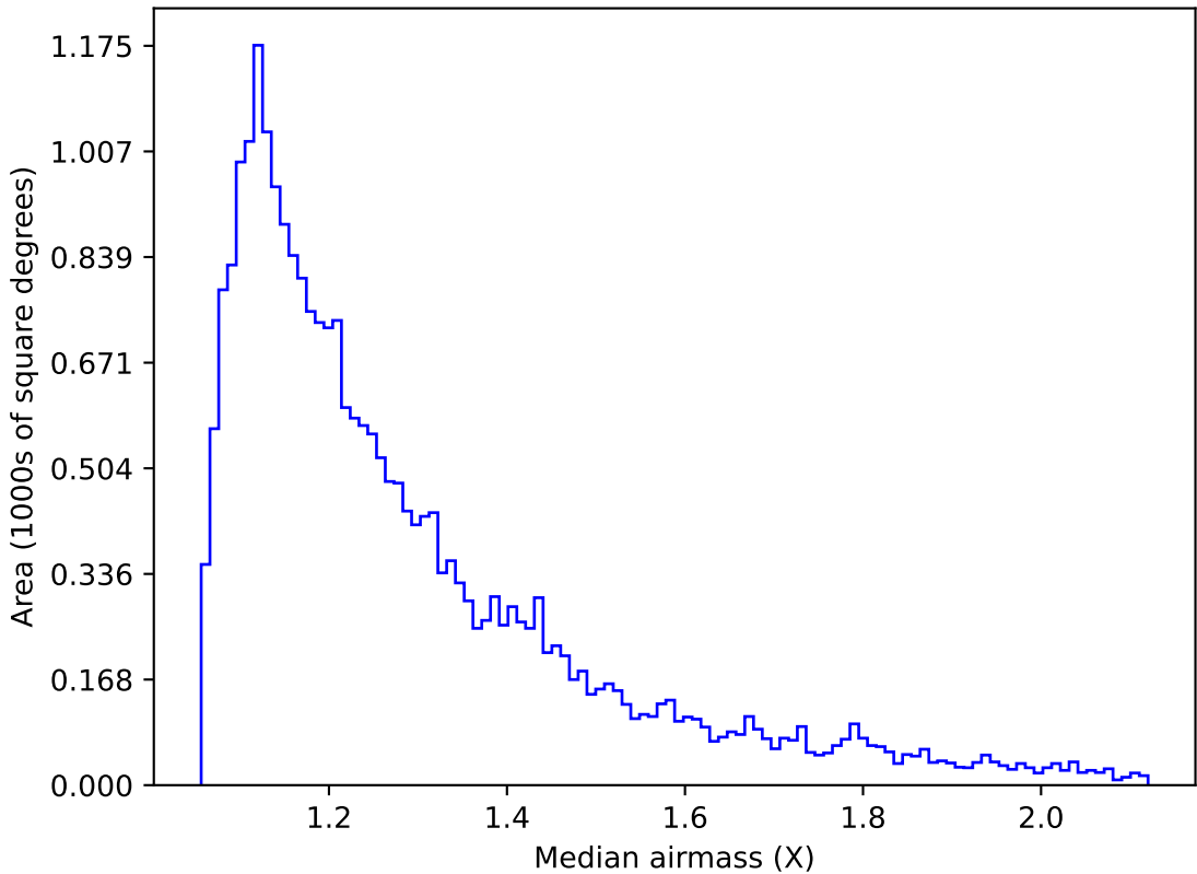
too_elab_r16_d3_gz_v3.4_10yrs Yr 1 g band: Median airmass
