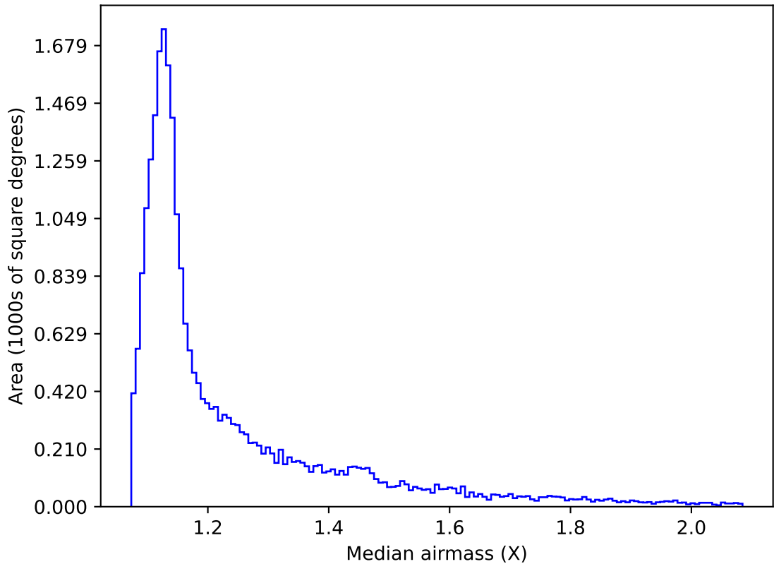
too_elab_r16_d3_gz_v3.4_10yrs Yr 1 all bands: Median airmass
