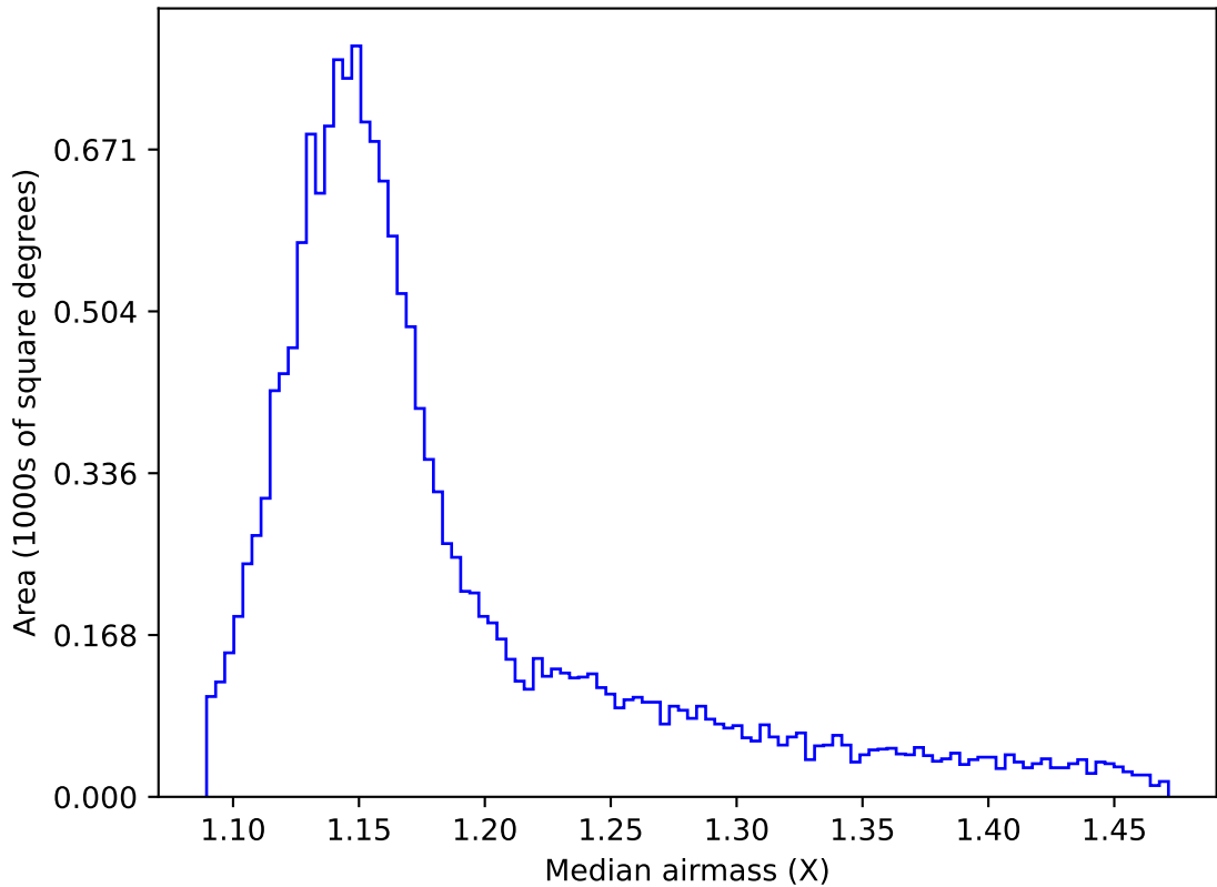
too_elab_r16_d3_gz_v3.4_10yrs WFD z band: Median airmass
