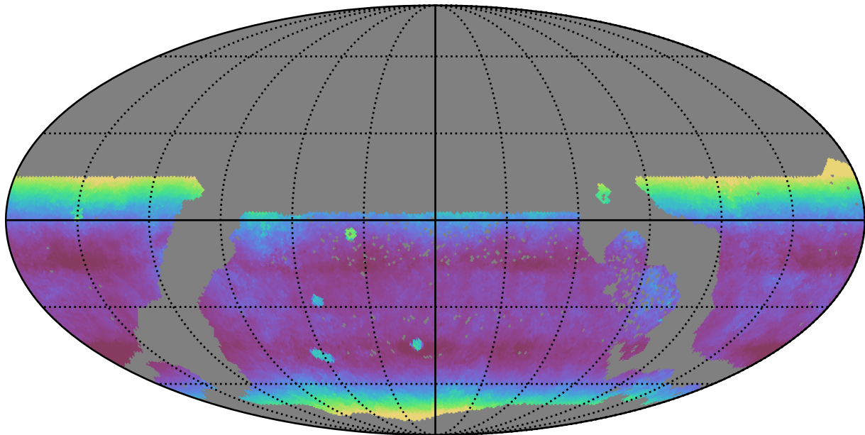
too_elab_r16_d3_gz_v3.4_10yrs WFD y band: Median airmass
