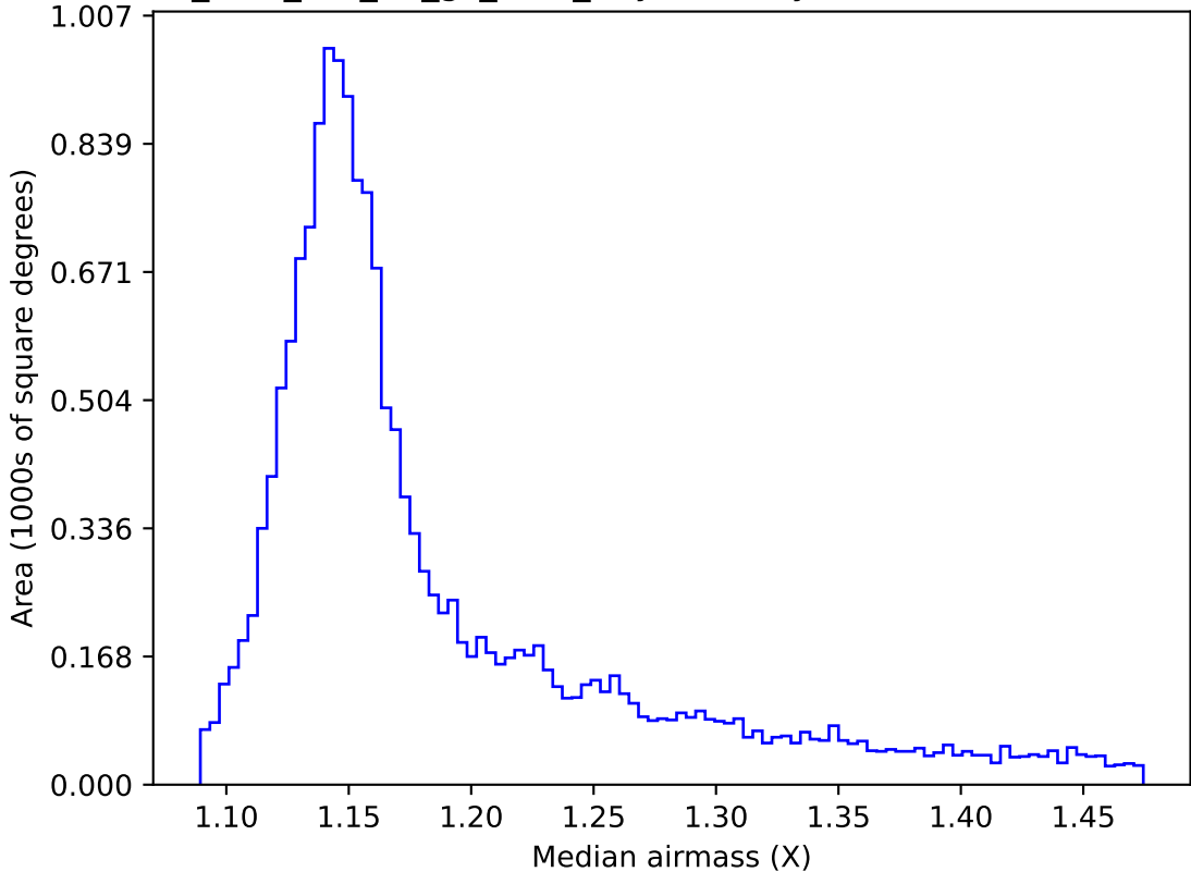
too_elab_r16_d3_gz_v3.4_10yrs WFD y band: Median airmass
