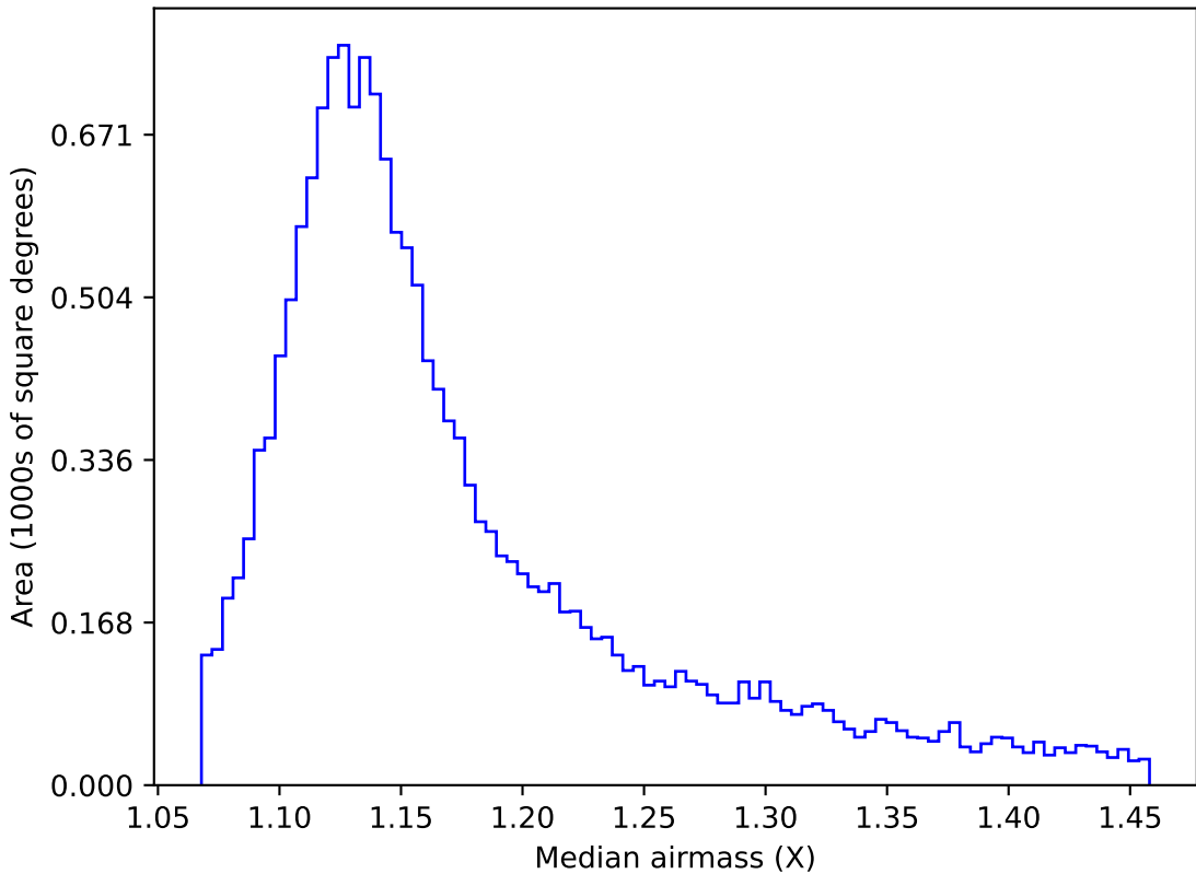
too_elab_r16_d3_gz_v3.4_10yrs WFD u band: Median airmass
