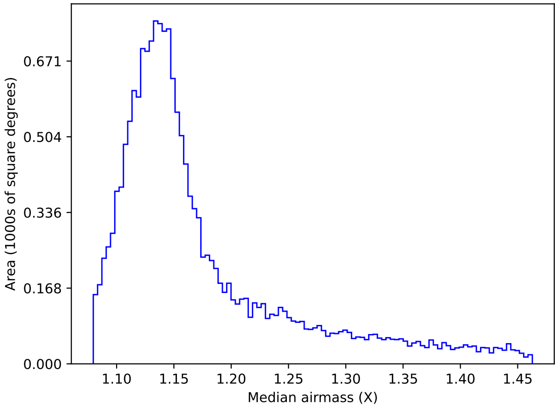
too_elab_r16_d3_gz_v3.4_10yrs WFD i band: Median airmass
