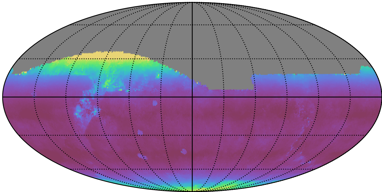
too_elab_r16_d3_gz_v3.4_10yrs All sky z band: Median airmass
