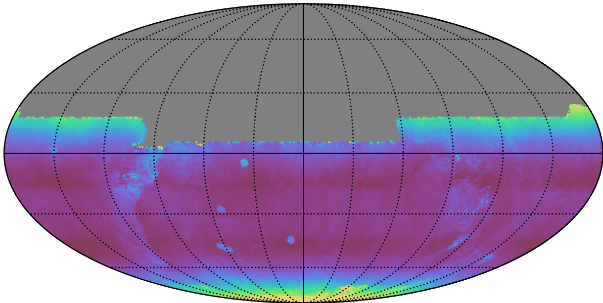
too_elab_r16_d3_gz_v3.4_10yrs All sky y band: Median airmass
