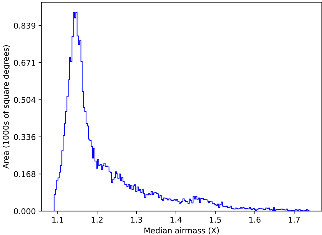
too_elab_r16_d3_gz_v3.4_10yrs All sky y band: Median airmass
